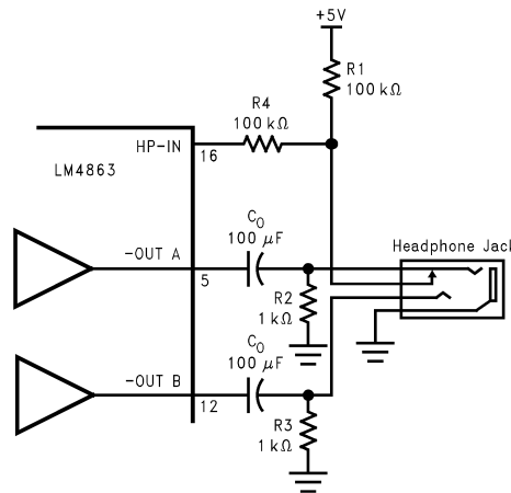
FIGURE 2. Headphone Circuit
