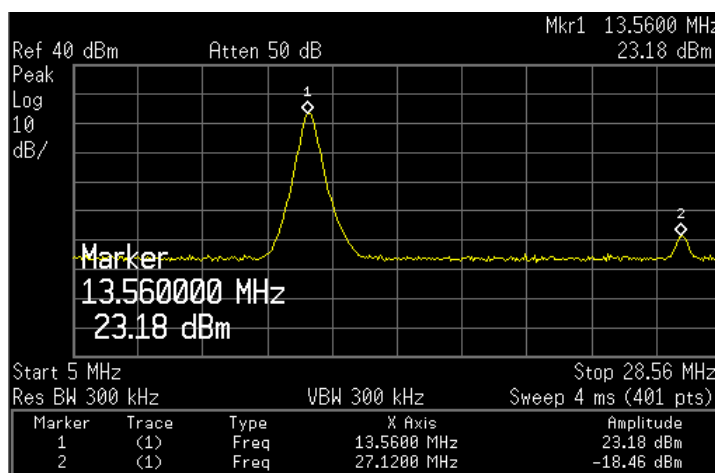
Figure 7. TRF7960A Out (Approximately +23 dBm)
