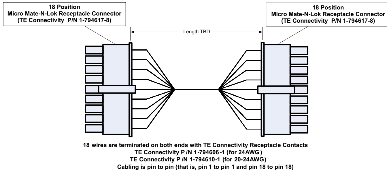
Figure 17. GPIO Cable Diagram
