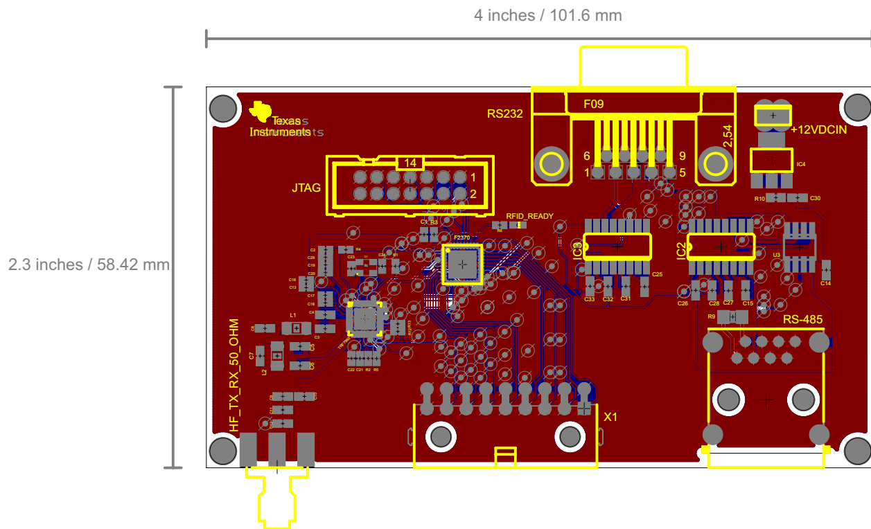
Figure 13. RFID Controller Board Layout
