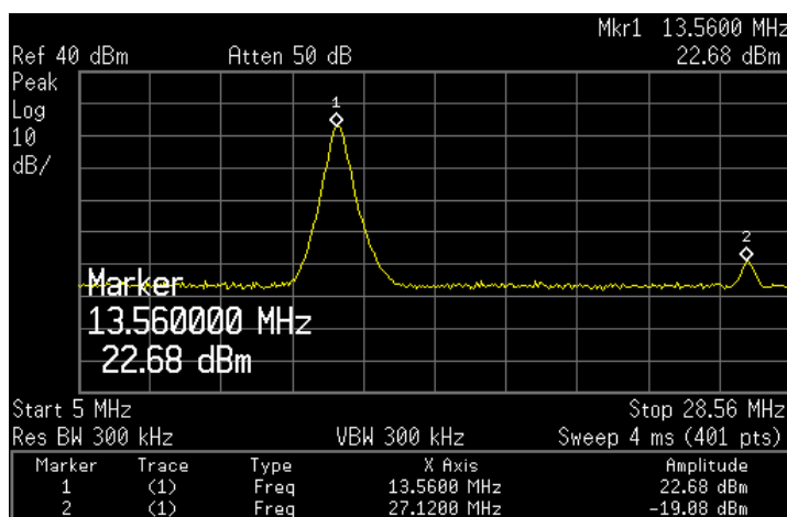
Figure 8. TRF7960A to PE42440 Out (Approximately 0.5-dBm Loss)
