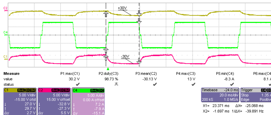
110Vac, 8A dynamic load to each rail
