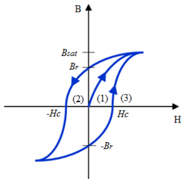
Fig. 3.2. Hysteresis loop
