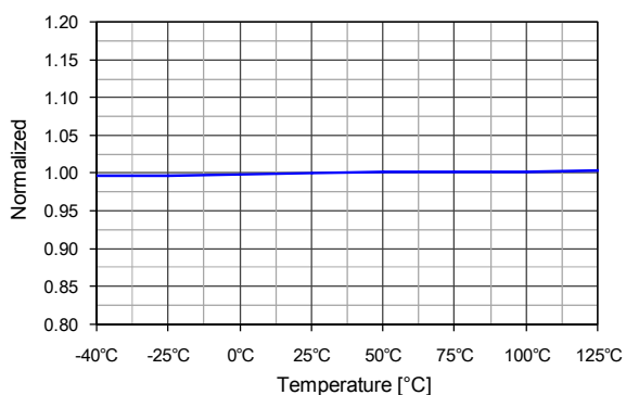
Figure 13. Shutdown Feedback Voltage ( V_{\text{SB}} ) vs. T_A
